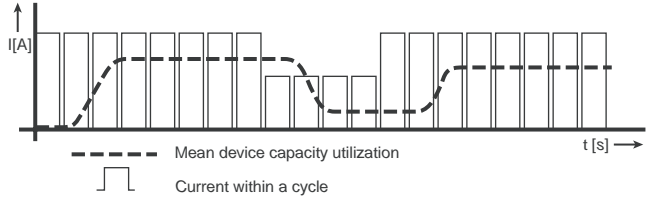
Figure 5.32 Mean device capacity utilization
