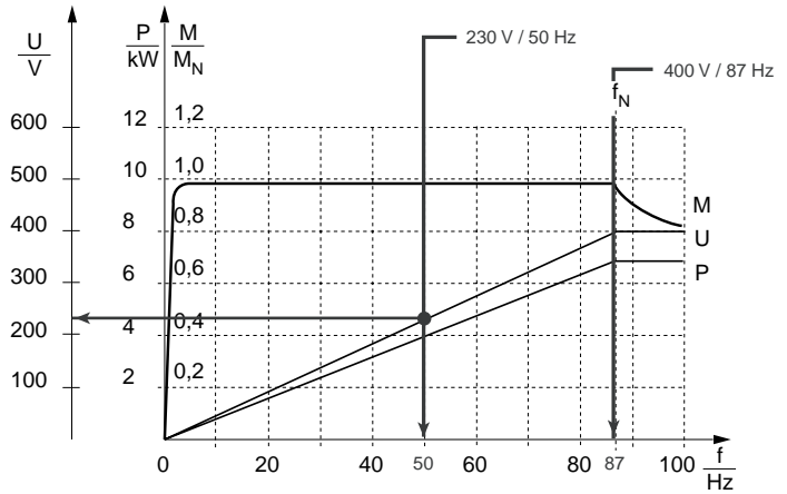
Figure 6.5 Constant torque range to 87 Hz
