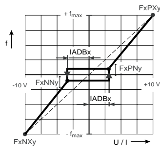
Figure 5.6 Backlash function in bipolar operation
