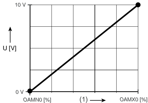
Figure 5.8 Scaling of the analog output
