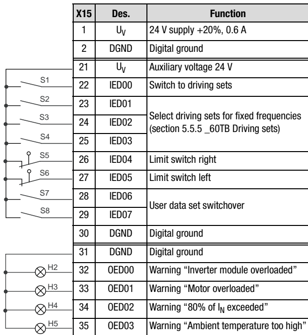
Figure 4.15 Assignment of control terminal expansion with ASTER = DRV_5
