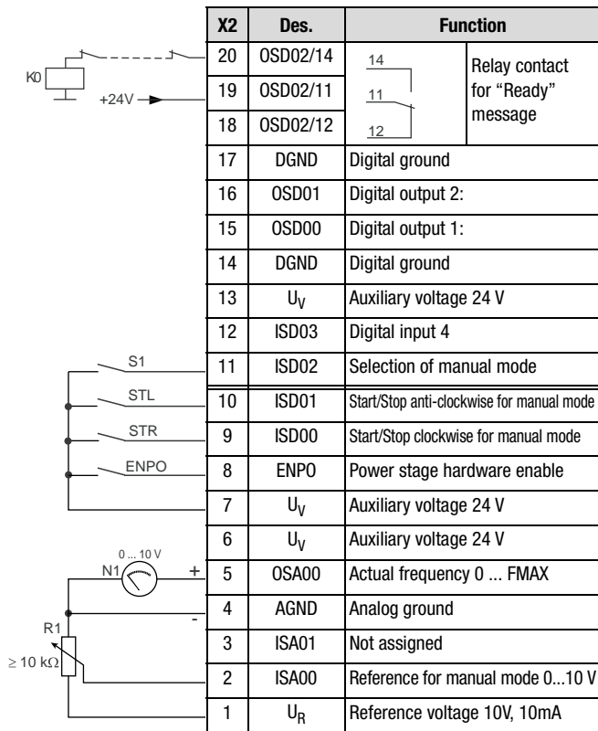
Figure 4.33 Control terminal configuration with ASTER=BUS_2
