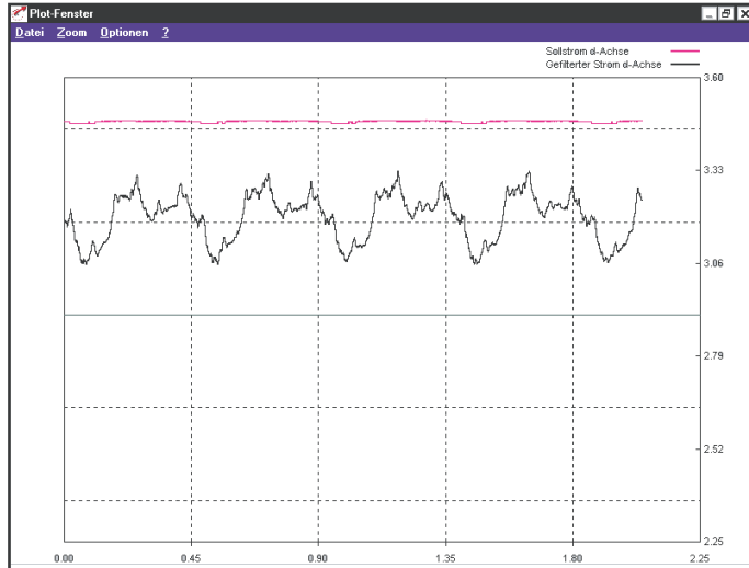
Figure 6.21 803-VCSFC = 199 %
