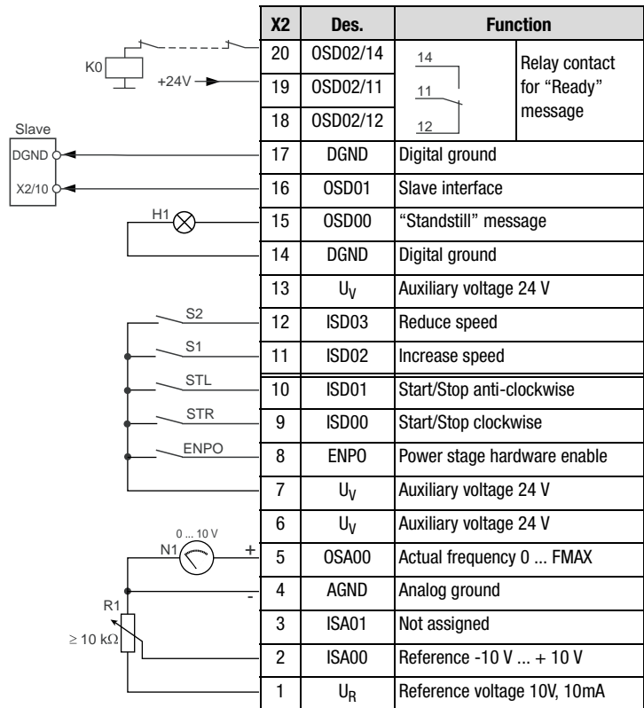
Figure 4.43 Control terminal assignment with ASTER = M-S_1
