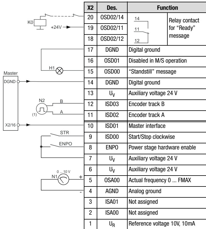
Figure 4.51 Control terminal assignment with ASTER = M-S_4
