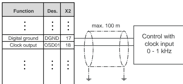
Figure 5.16 Wiring when using the clock output
