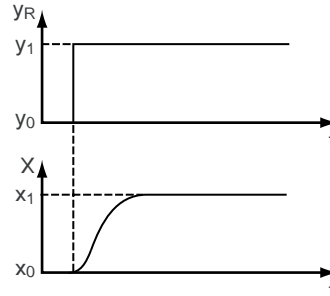
Figure 5.59 Step response of a higher-order controlled system
