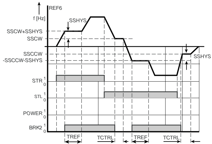
Figure 5.36 Function of motor holding brake BRK2 in VFC (SFC)
