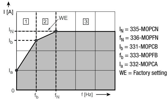
Figure 5.26 Characteristic adjustment by interpolation points below the rated frequency f_N
