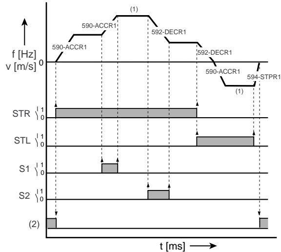
Figure 4.44 Example of a driving profile for two directions of rotation (ASTER=M-S_1)
