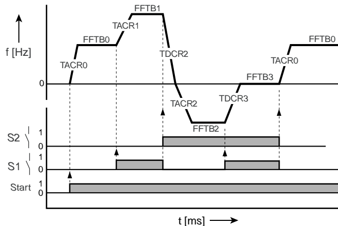
Figure 5.43 Example of driving sets with fixed frequencies
