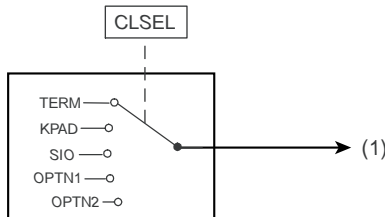
Figure 5.20 Function block: Control location selector
