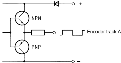
Figure 6.28 HTL output configuration block diagram
