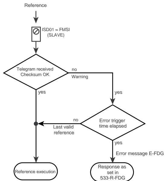
Figure 5.47 Structure of reference processing in the slave
