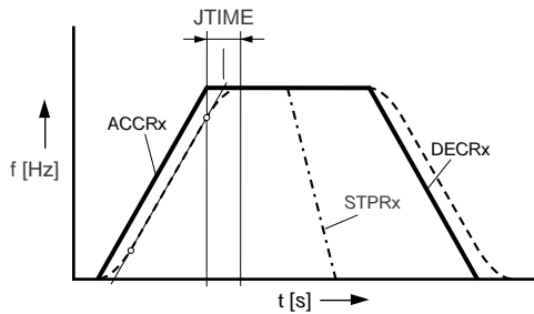
Figure 5.41 Driving profile of ramp generator
