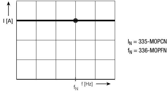
Figure 5.25 Factory setting of the motor protection characteristic
