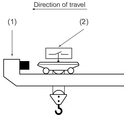
Figure 5.10 Limit switch evaluation
