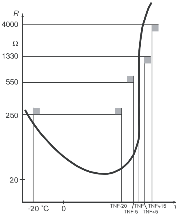
Figure 5.23 Resistance diagram as function of temperature of a DIN PTC
