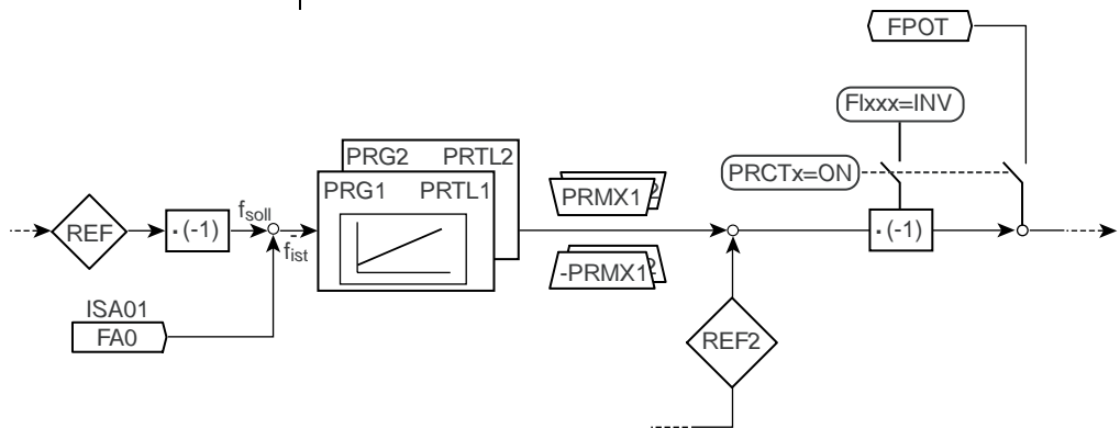
Figure 5.53 Block diagram of process controller with integration into reference structure
