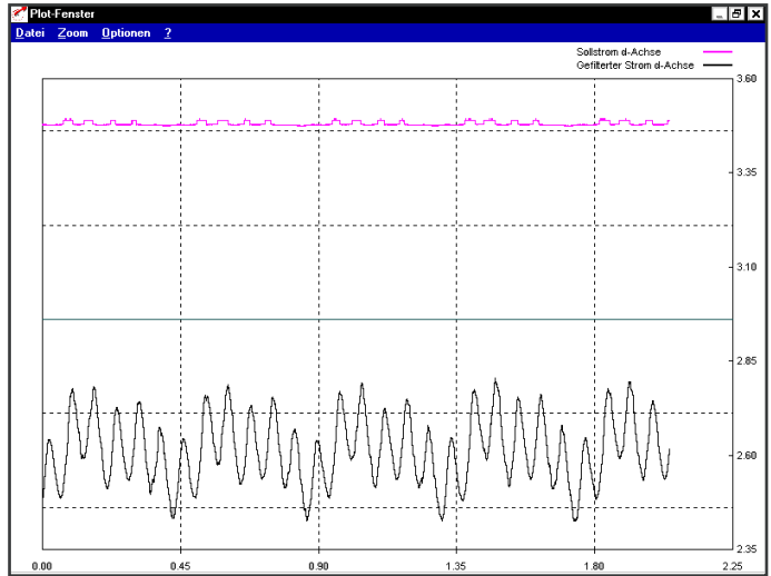
Figure 6.22 803-VCSFC = 0 %
