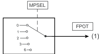
Figure 5.38 Function block: MOP function selector
