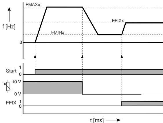
Figure 5.21 Limitation of output frequency
