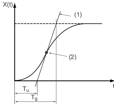
Figure 5.60 Graphical definition of delay and compensating times
