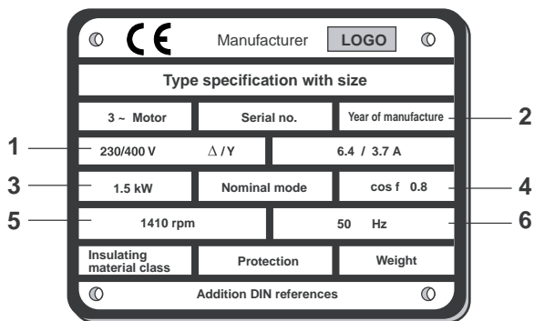
Figure 5.1 Motor rating plate
