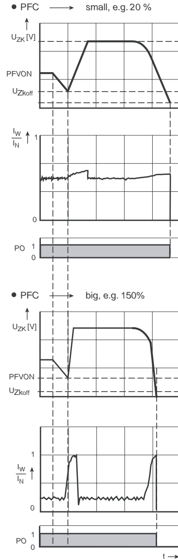
Figure 5.28 Effect of effective current reference PFC
