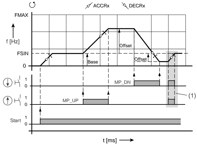
Figure 5.39 Basic function with reset to base value (corresponds to setting F1 in Table 5.80)
