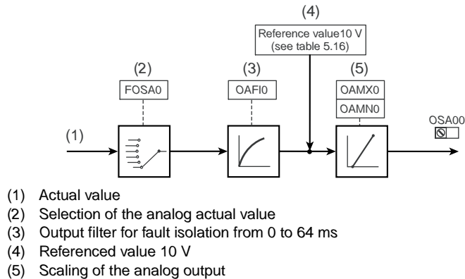
Figure 5.7 Function block for adaptation of the analog output
