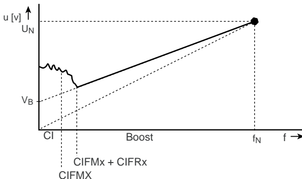
Figure 6.13 Combination of current injection and boost voltage
