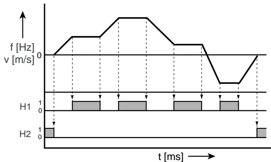
Figure 4.18 Example of a driving profile for two directions of rotation (ASTER=ROT_1)
