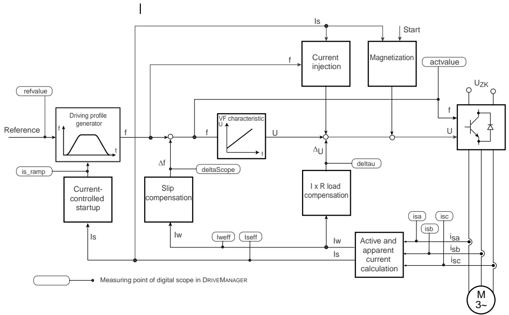
Figure 6.11 Block diagram of control circuit (VFC)
