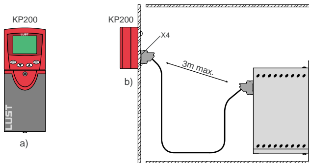
Bild 3.3 Mounting the KEYPAD: a) on the CDA3000 inverter module (connector X4) or b) on the switch cabinet door
