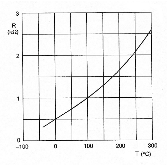
Figure 5.22 Resistance diagram as function of temperature of a PTC KTY 84-130
