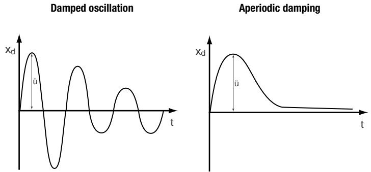
Figure 5.57 Control characteristic with damped oscillation
