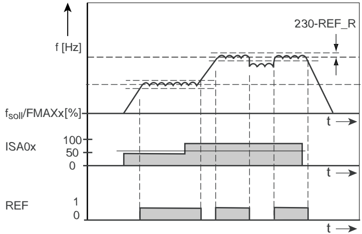
Figure 5.12 Digital output with “reference reached” setting when using the “reference-reached window”
