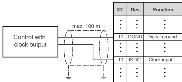
Figure 5.14 Wiring with reference input via clock input
