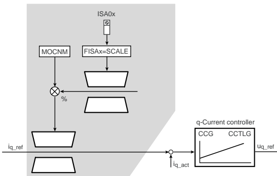
Figure 6.30 FOR current controller
