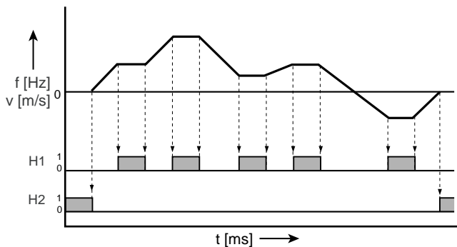
Figure 4.49 Example of a driving profile with Master/Slave coupling (ASTER = M-S_3)
