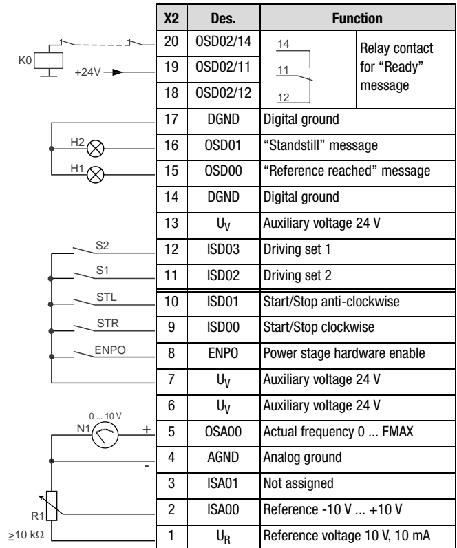
Figure 4.29 Control terminal assignment with ASTER = ROT_6
