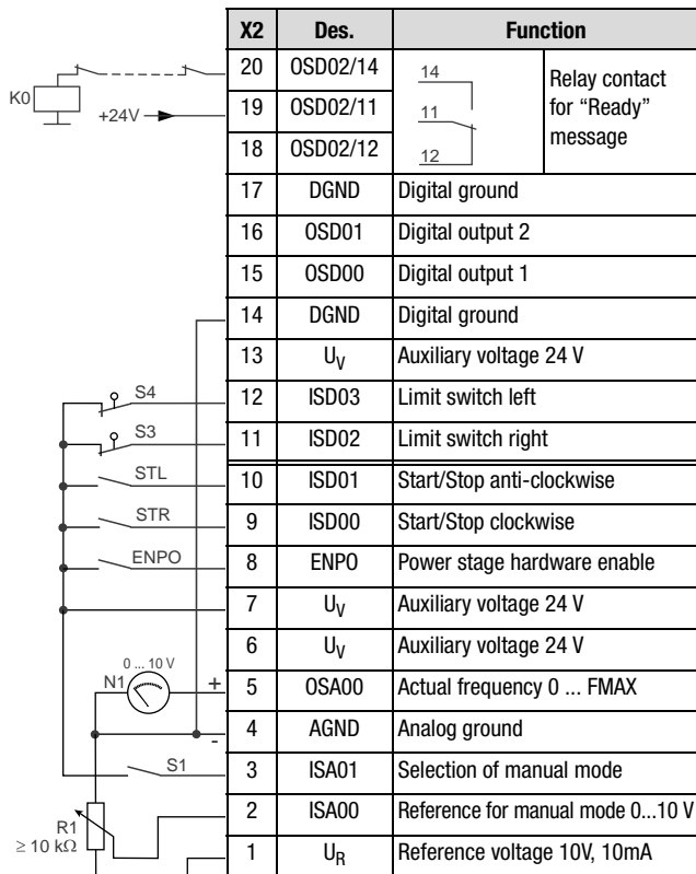
Figure 4.35 Control terminal configuration with ASTER = BUS_3
