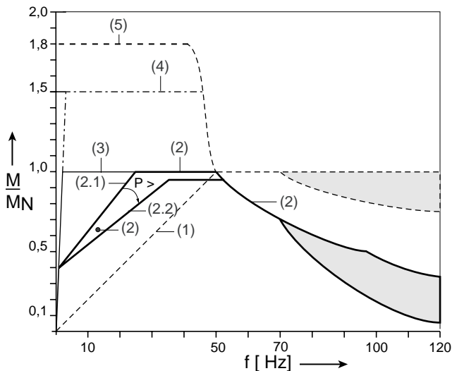
Figure 5.27 Typical torque characteristic of a standard three-phase AC motor
