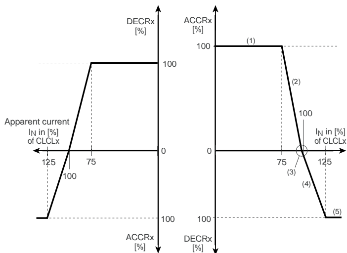
Figure 5.51 Dependency of the ramp steepness on the rated device current dimensioned to the current limit value
