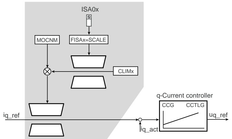
Figure 6.19 SFC current controller
