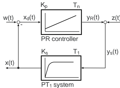
Figure 5.54 Presentation of a control circuit
