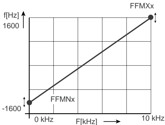
Figure 5.15 Scaling of clock input ISD01
