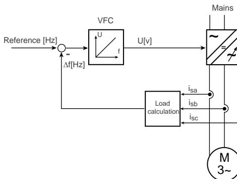
Figure 6.10 Anti-pendulum block diagram
