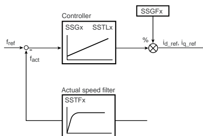
Figure 6.18 SFC speed controller
