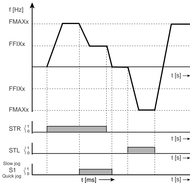
Figure 5.42 Fixed frequency for quick jog/slow jog application
