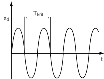
Figure 5.56 Control characteristic at stability limit
