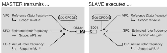
Figure 5.46 Reference coupling dependent on chosen operation mode on the master
