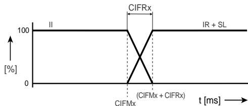
Figure 6.2 Combination of voltage frequency control functions
