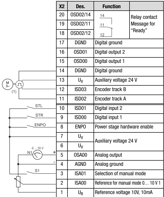
Figure 4.38 Control terminal configuration with ASTER = BUS_5
