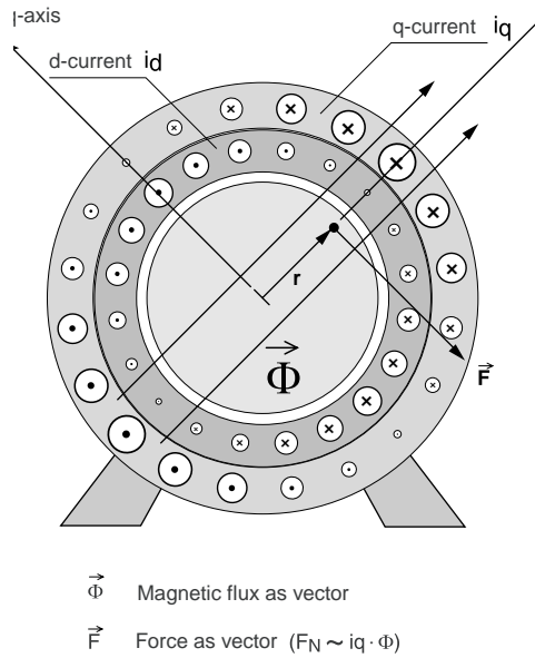
Figure 6.16 Principle of function of the asynchronous motor
