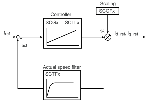
Figure 6.29 FOR speed controller
