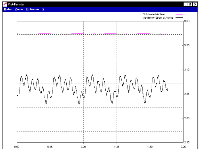
Figure 6.23 803-VCSFC = 68 % after calculation by auto-tuning
