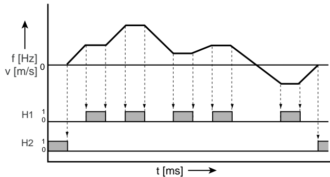
Figure 4.44 Example of a driving profile for two directions of rotation (ASTER=M-S_1)
