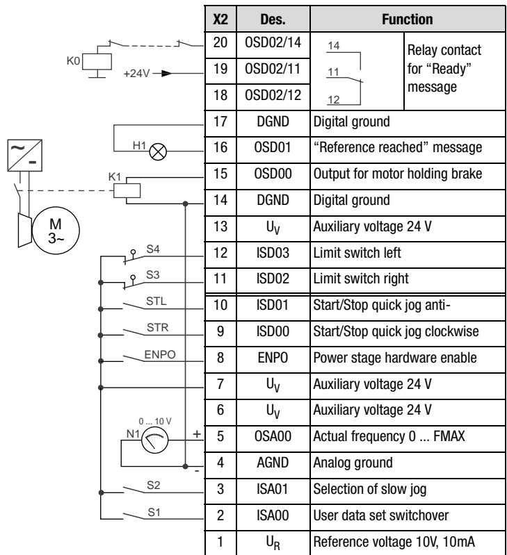
Figure 4.7 Control terminal assignment with ASTER = DRV_3
