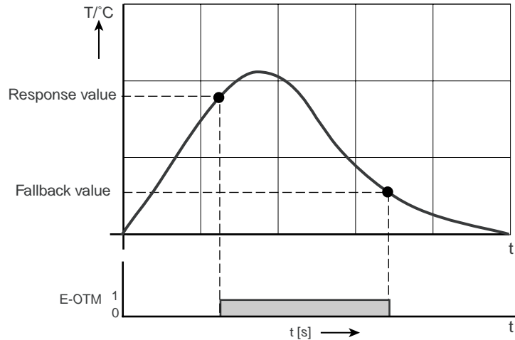
Figure 5.24 PTC evaluation operation diagram
