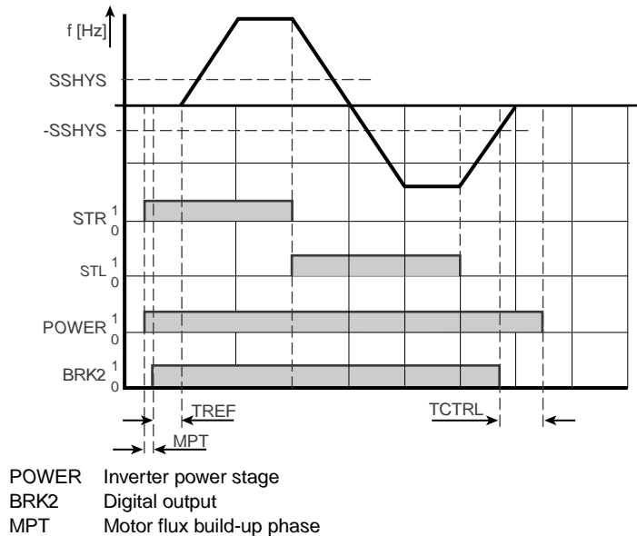
Figure 5.37 Function of motor holding brake BRK2 in control mode FOR
