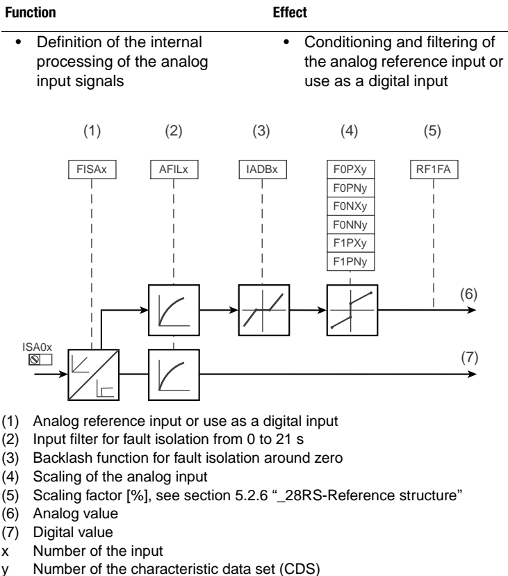
Figure 5.4 Function block for adaptation of the analog inputs
