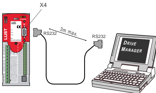
Bild 3.8 Connection via RS232 interface cable (9-pin, plug-and-socket)
