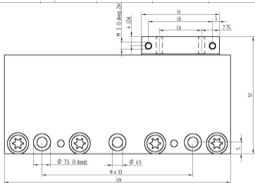
Dimensions of Coilant
