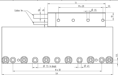
Dimensions of Coils
