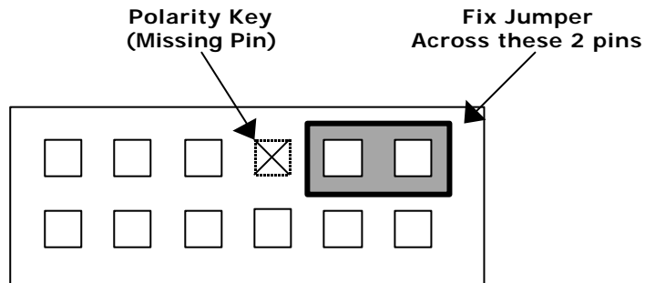
Fig.1 - Emulator Header
