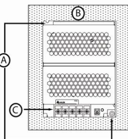
Base Mounting
